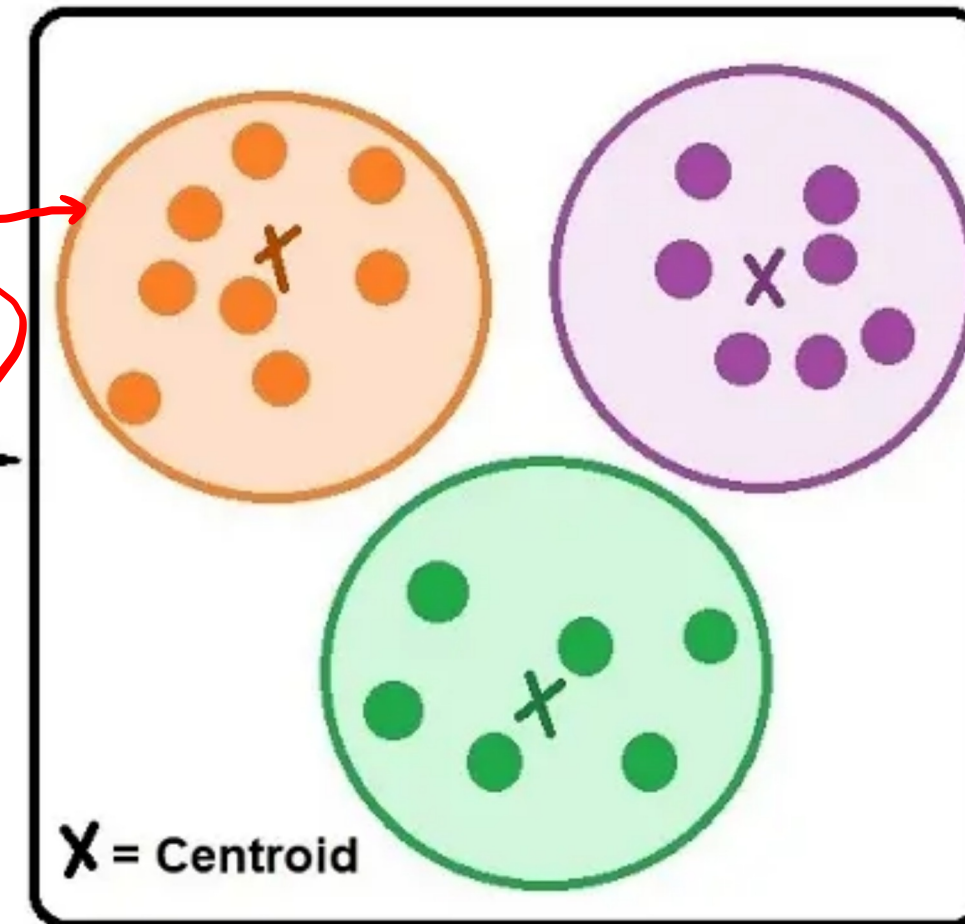
Labeled Clusters
