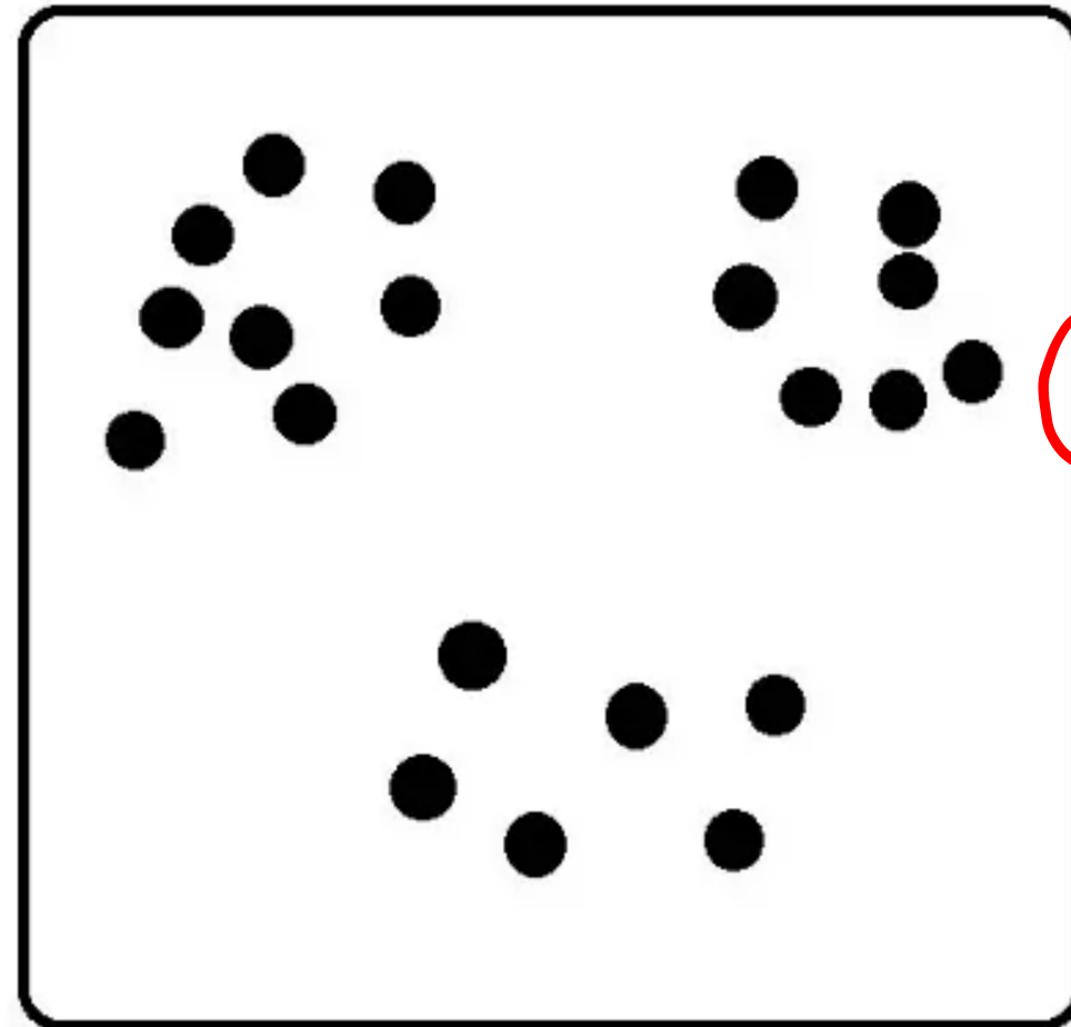
Unlabeled Data
