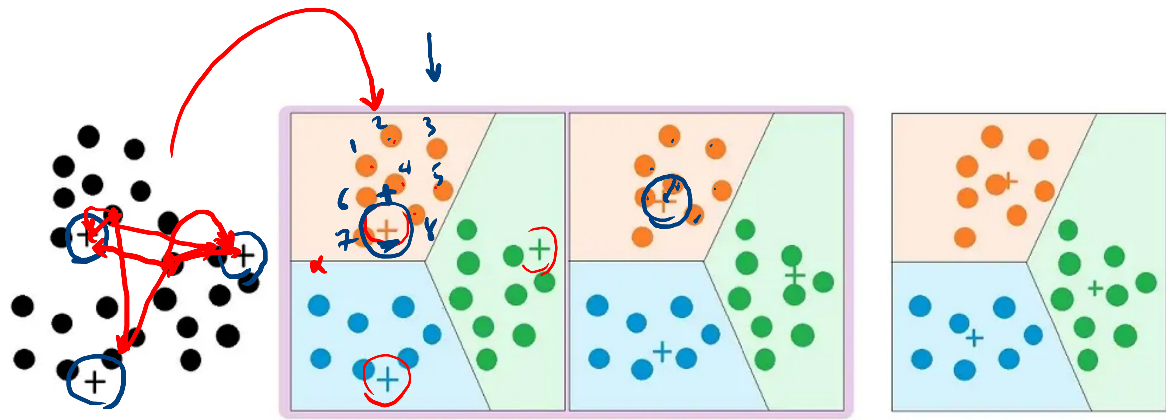
Means Initialization → Assignment of Clusters → Means Update → Convergence
